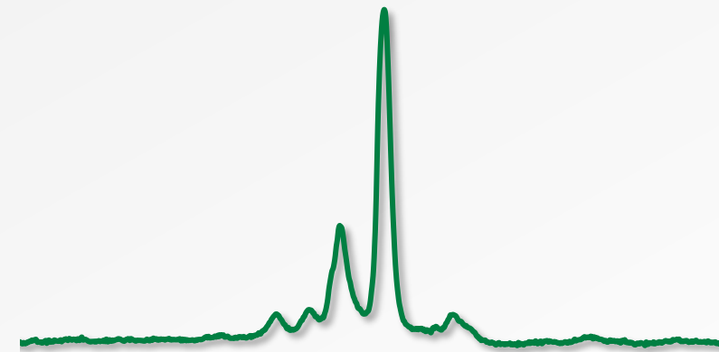
UH + HR AESlytes
