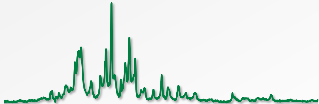
Ultra-High Resolution (UH) AESlytes
