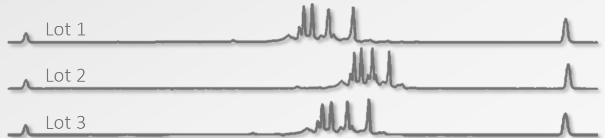
Traditional Carrier Ampholytes
