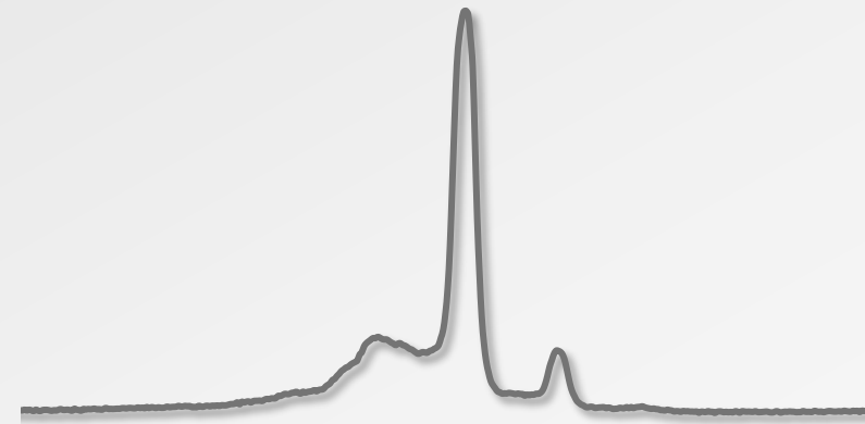
Traditional Carrier Ampholytes
