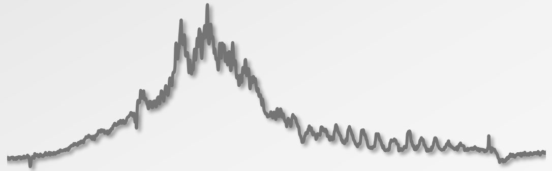
Traditional Carrier Ampholytes
