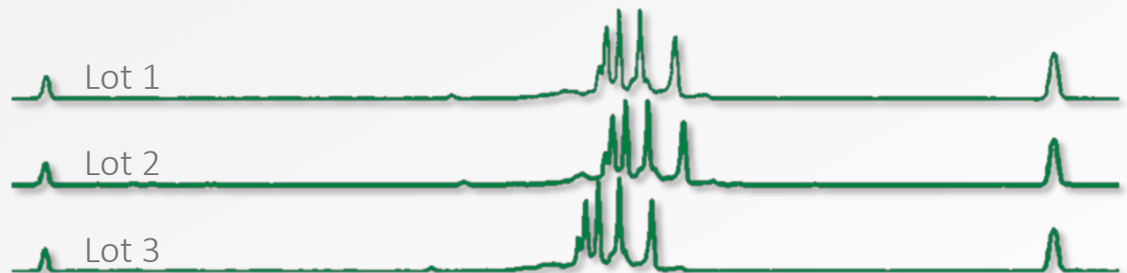
High Resolution (HR) AESlytes
